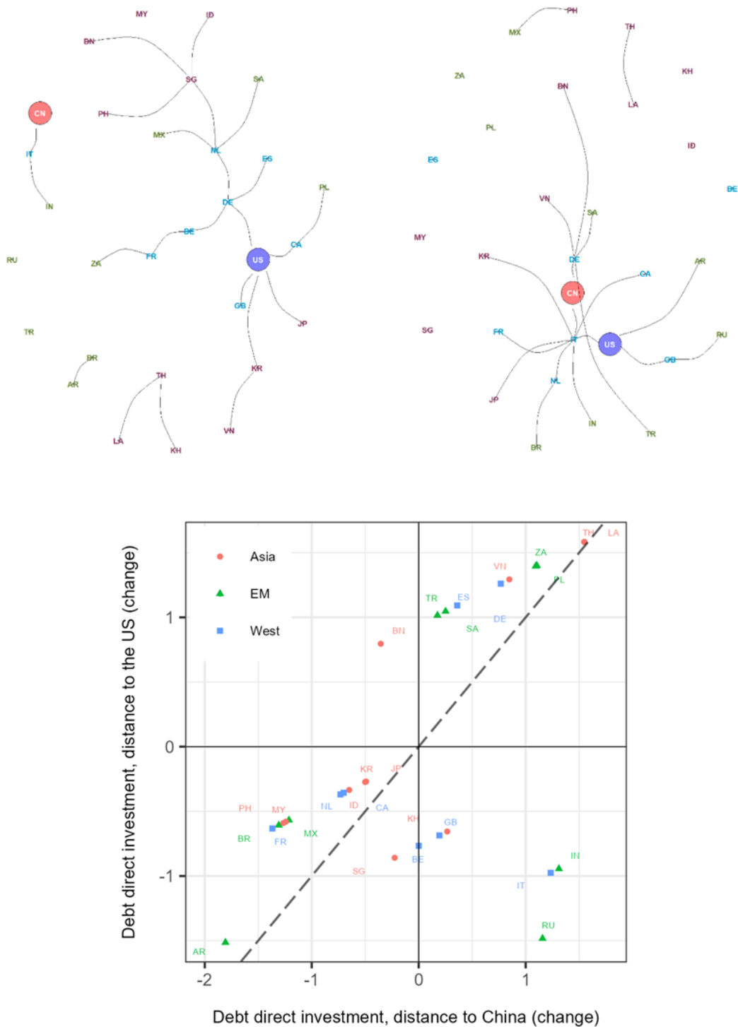
Figure A2.4.4. Minimum spanning trees and distance changes: debt foreign direct investment, ultimate investor basis 2013–2017 2018–2022
